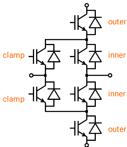
Example of a 3-level ANPC
