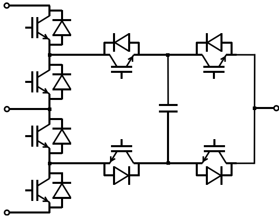
Example of a 5-level Multilevel ANPC
